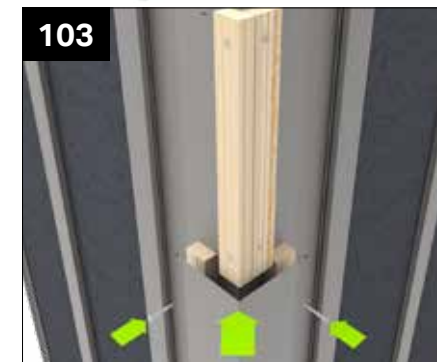
103 If a structural post has been specified, the batten arrangement is altered, and a steel angle is used to allow for the cement board to be easily fitted and reinforce the corner.
