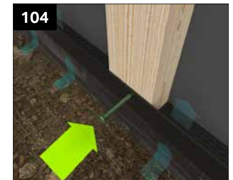
104 At the base of the wall attach the perforated ventilation trim to the battens. This allows for ventilation and drainage but inhibits vermin/insects.
