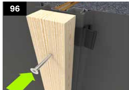
96 Position a 25mm batten, treated timber (optionally provided) or alternative, against the clips trapping the membrane in place. At apertures this batten is positioned inline with the opening. Secure the batten to the walling full and half clips using the winged fixing screw (provided with battens).
